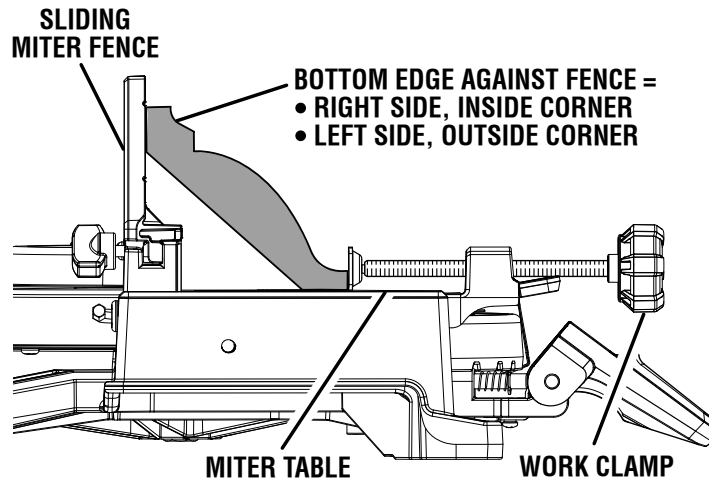
LARGE CROWN MOLDING NESTED AGAINST REAR FACING MITER FENCE
