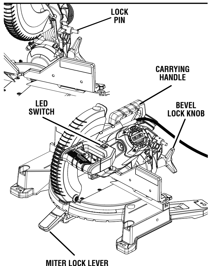
SAW ARM LOCKED IN DOWN POSITION
