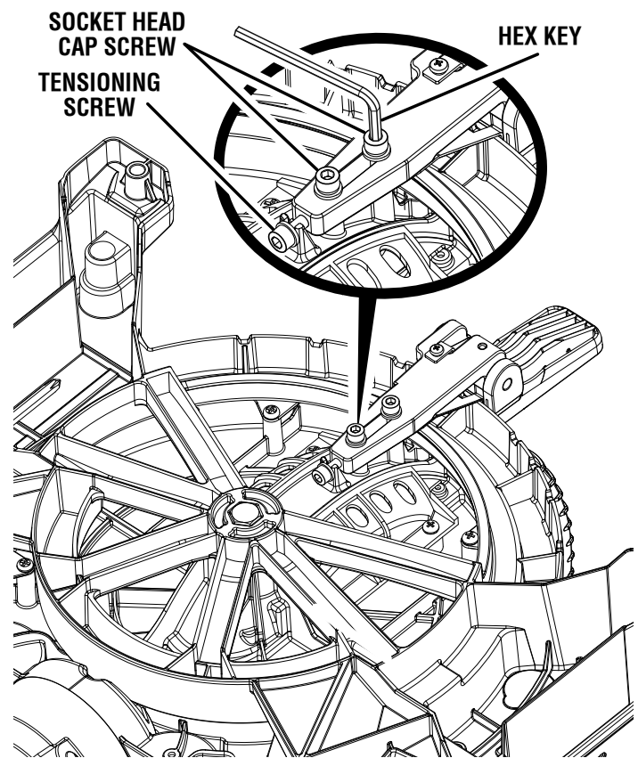
BOTTOM VIEW OF SAW
