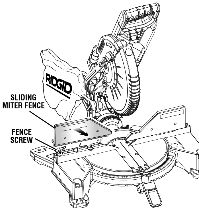
VIEW OF SAW FROM FRONT WITH FENCES FACING FORWARD
