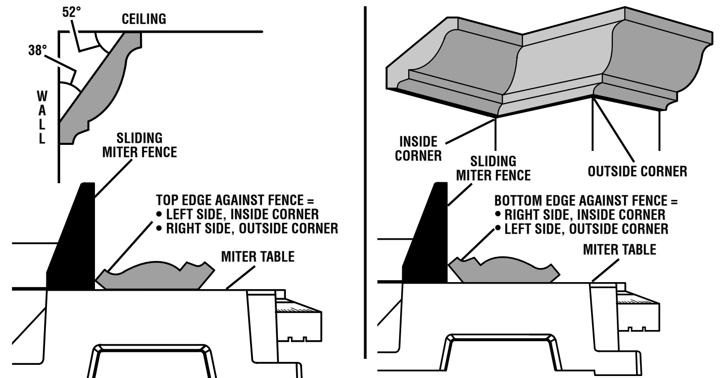
CROWN MOLDING FLAT ON MITER TABLE
