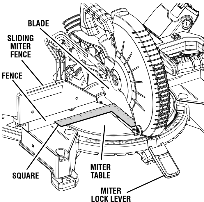
VIEW OF BLADE SQUARE WITH FENCE Fig. 14
