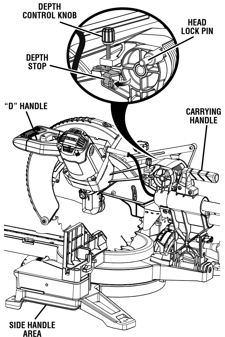
SAW ARM LOCKED IN DOWN POSITION
